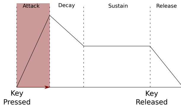
Figure 284: Attack on ADSR Envelope
